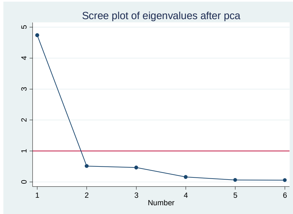
Figure 1: Scree plot for PCA generated composite WGI index Source: Author's calculation based on appropriate data
