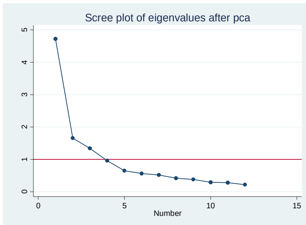
Figure 2: Scree plot for PCA generated composite ICRG index Source: Author's calculation based on appropriate data
